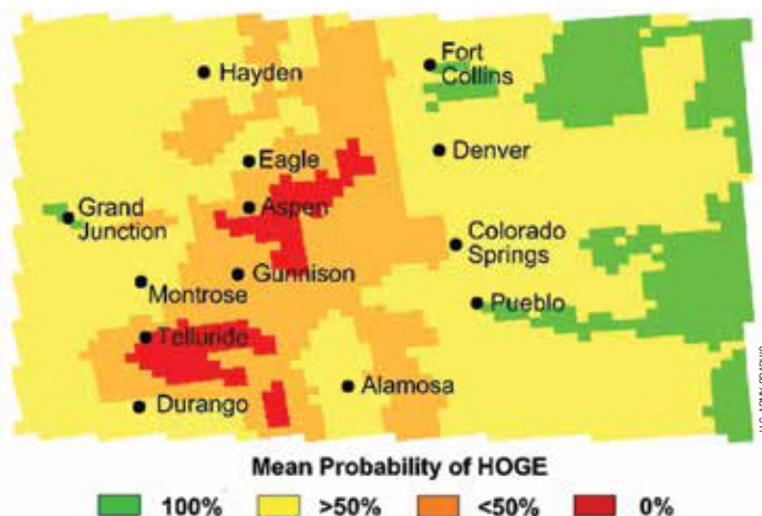
Cumulative probability of Hover Out of Ground Effect (HOGE) capability in Colorado during an average July for a representative 1970s-era attack helicopter design at primary design mission gross weight and ordnance loadout.
